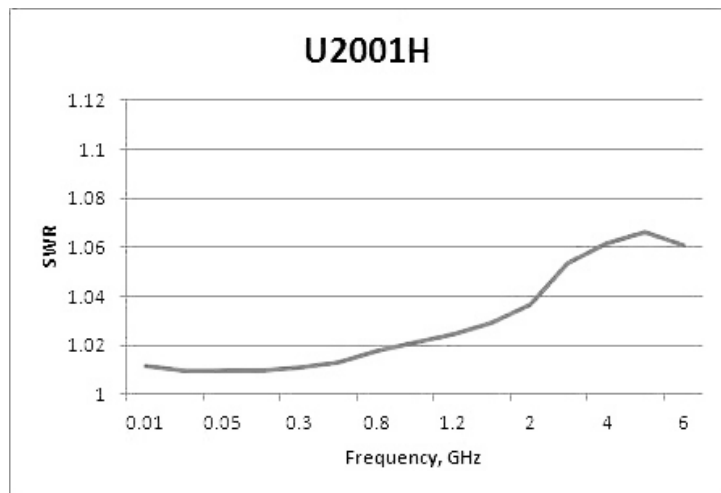
Typical SWR for U2001H sensor ( 25\text{ }^{\circ}\text{C} \pm 10\text{ }^{\circ}\text{C} )
