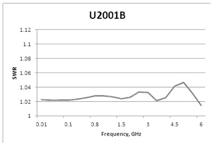
Typical SWR for U2001B sensor ( 25\text{ }^{\circ}\text{C} \pm 10\text{ }^{\circ}\text{C} )
