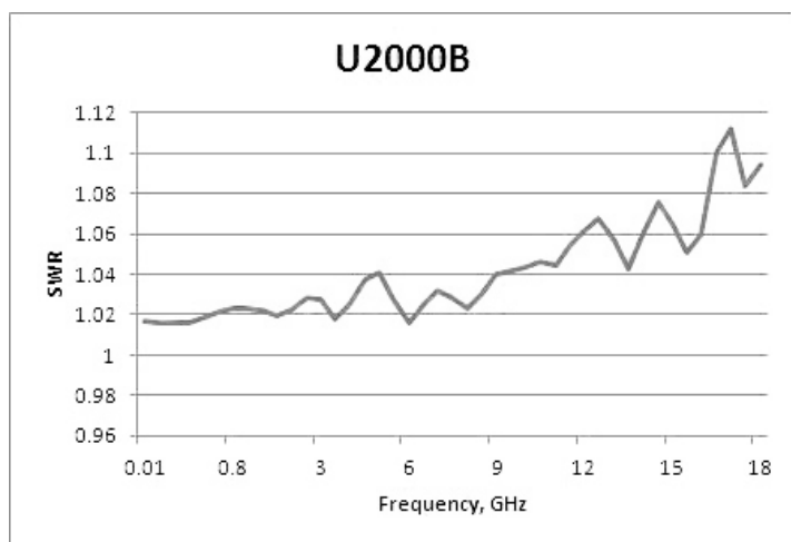
Typical SWR for U2000B sensor ( 25\text{ }^{\circ}\text{C} \pm 10\text{ }^{\circ}\text{C} )
