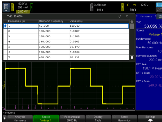
Figure 9. Harmonic measurements with graph
