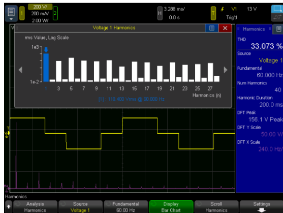
Figure 11. Harmonic measurements with bar graph
