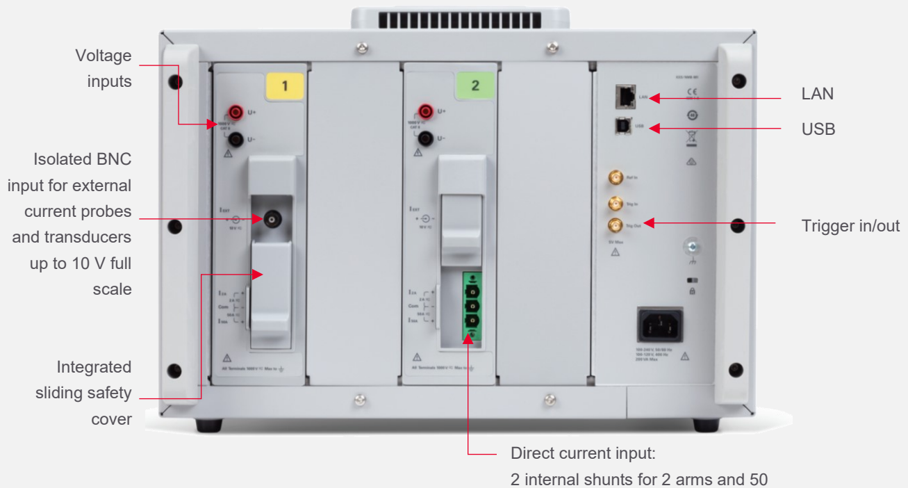
Figure 16. Rearview of PA2201A
