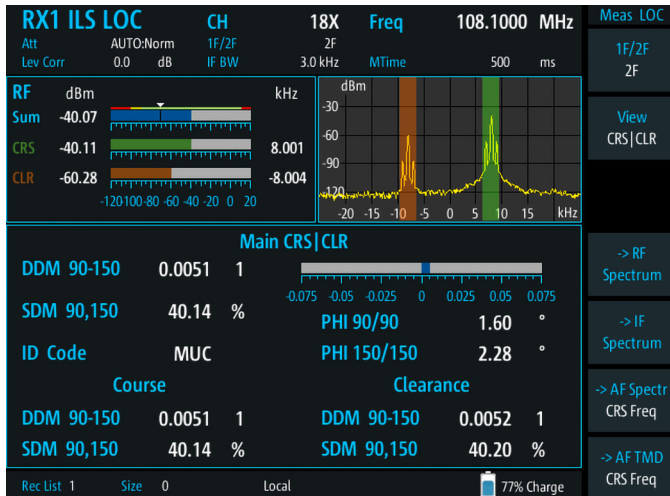
Measurement of a 2F ILS installation
