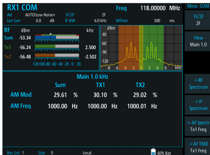
Analysis of communications signals
